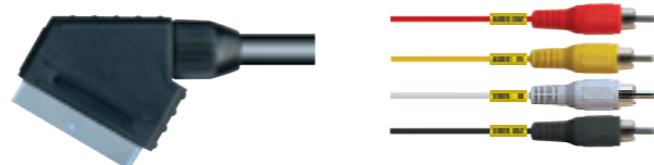
SC1012 21 PIN scart plug to 6 RCA plugs cable A:OD 8.5mm B:OD 9mm C:OD 2.6×10.4mm+2.6×5.2mm
